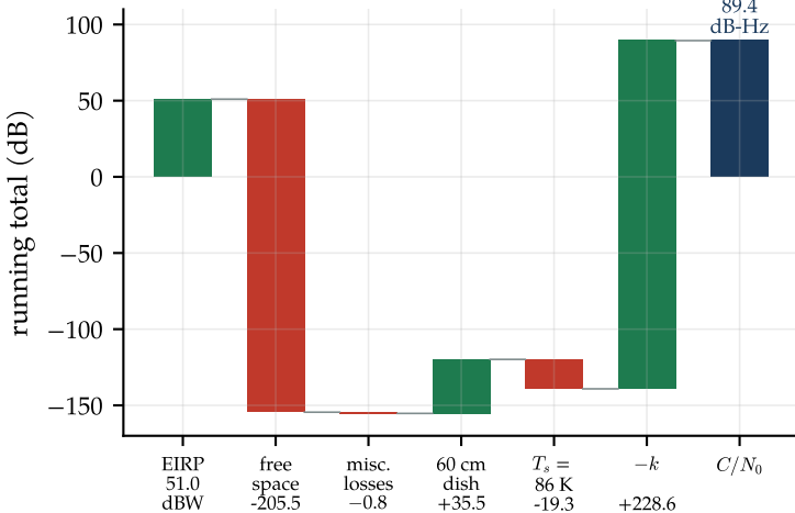
downlink C/N_0 build-up
