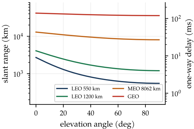
slant range and delay
