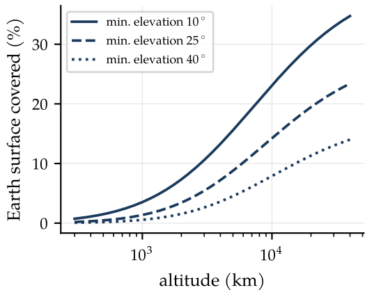
one satellite's coverage
