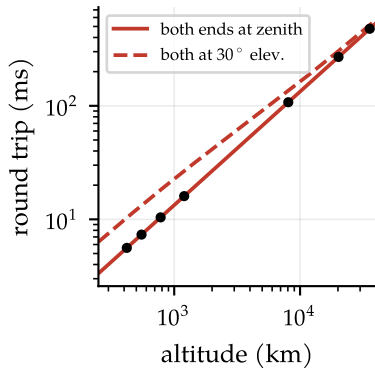
bent-pipe round-trip time
