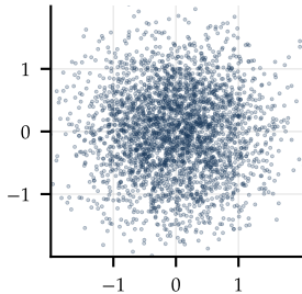
received (80 km CD)
