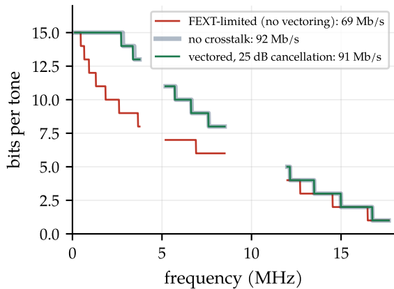
VDSL2 17a downstream, 600 m, 20 disturbers
