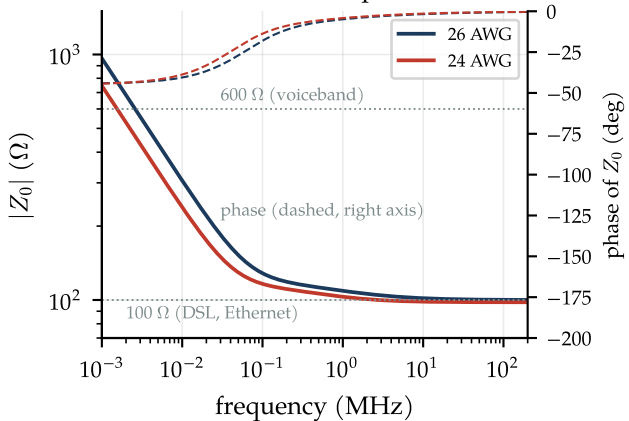
characteristic impedance
