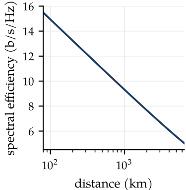
nonlinear Shannon limit
