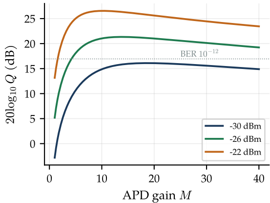
an optimum avalanche gain
