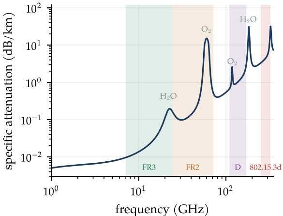
(a) clear air, sea level, 7.5 \text{ g/m}^3 (approx.)
