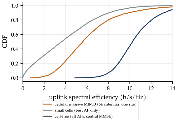
(b) per-user SE, 16 users, perfect CSI
