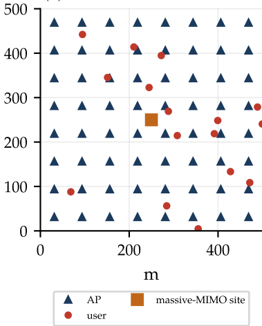
(a) 64 APs vs one 64-antenna site
