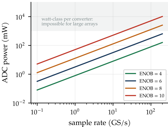
(a) Walden FOM = 50 fJ/conv.-step
