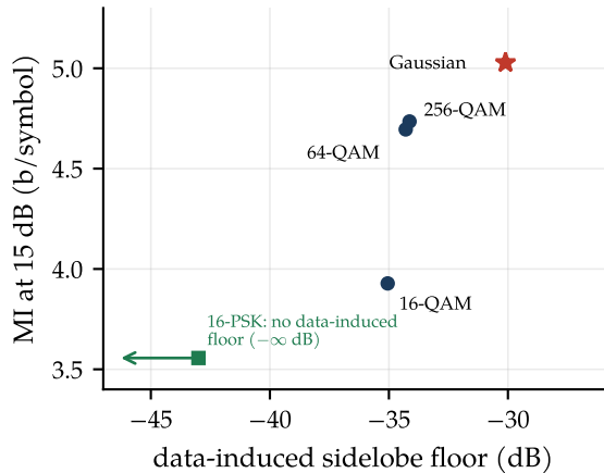
(b) the deterministic--random trade-off
