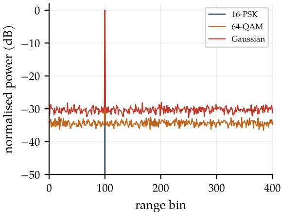
(a) correlation receiver, N = 1024
