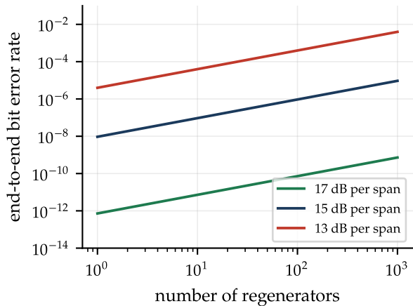
Digital: errors grow only linearly
