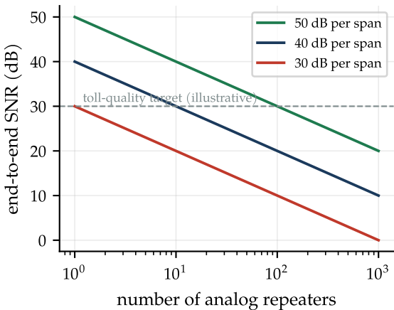
Analog: noise accumulates
