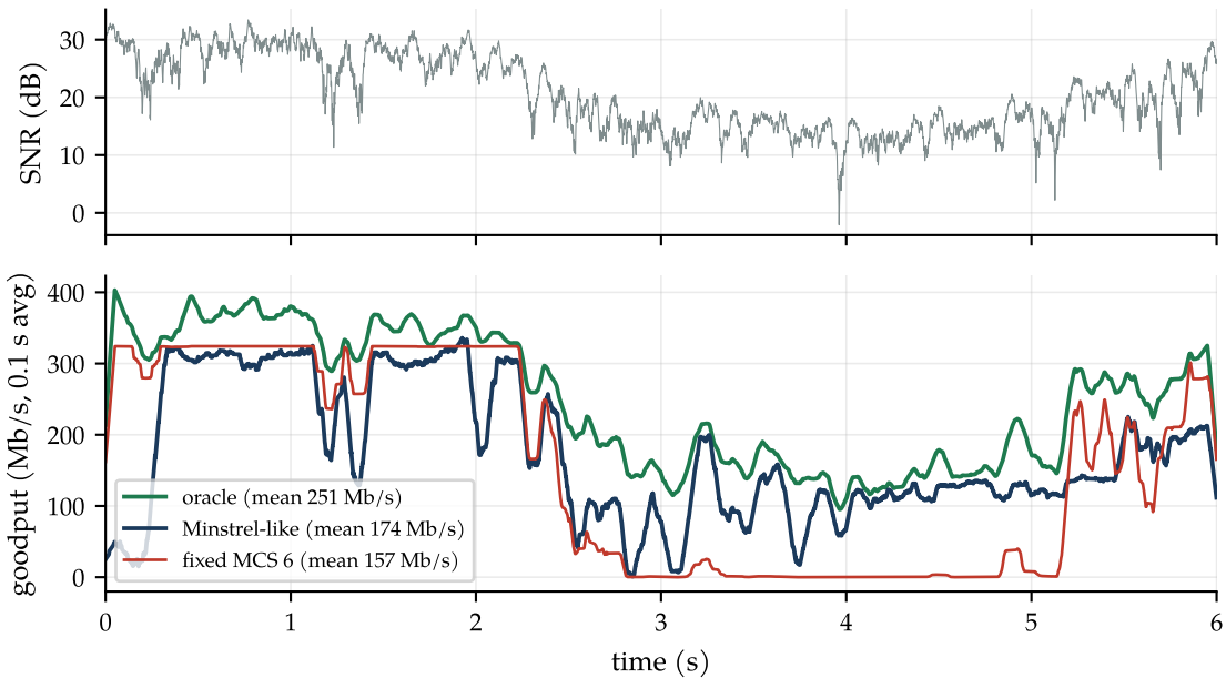
Channel seen by a moving station (80 MHz, one stream)
