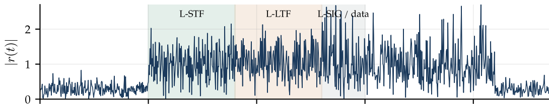
Received 802.11 legacy preamble: multipath, 80 kHz CFO, SNR 10 dB
