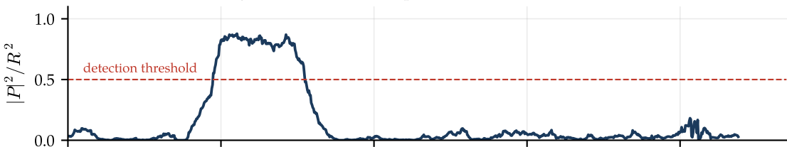
Delay-16 autocorrelation (packet detection, AGC window)
