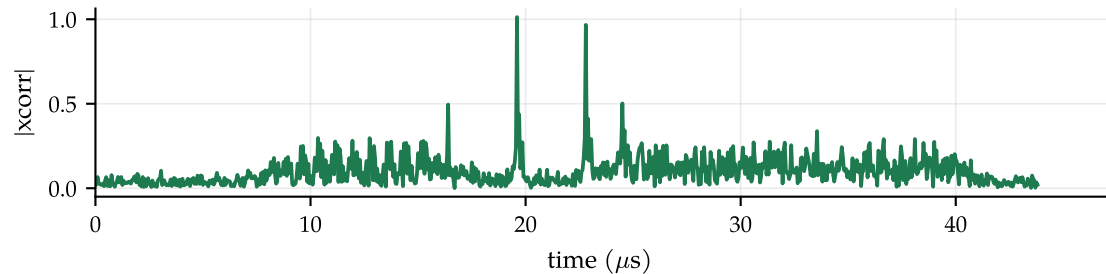
Cross-correlation with the known L-LTF symbol (fine timing); coarse CFO estimate 76.5 kHz
