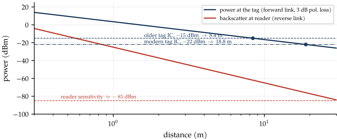
UHF RFID at 915 MHz, 4 W EIRP: the forward link limits range
