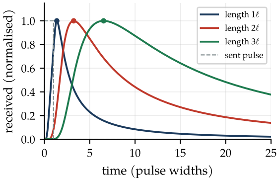
One pulse, three cable lengths
