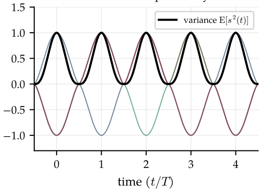
Statistics that repeat every T
