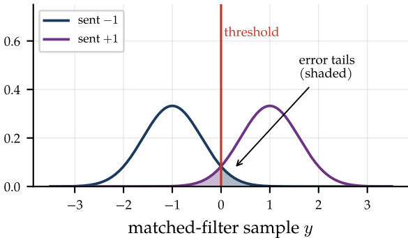
equal priors: threshold at the midpoint
