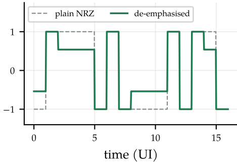
Transmitter output
