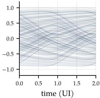
eye, plain
