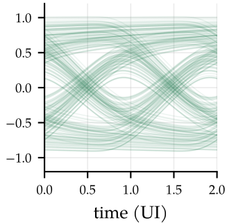
eye, de-emphasised
