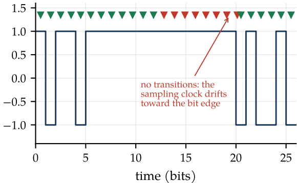
Clock starvation
