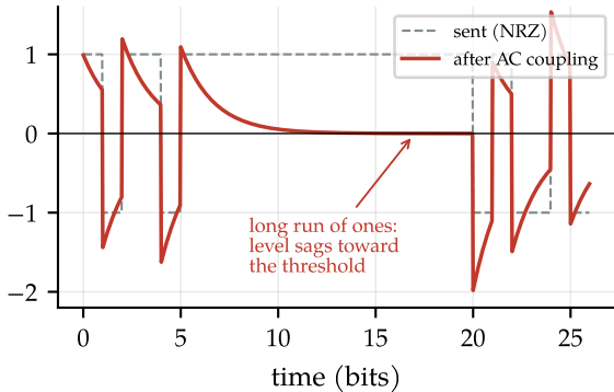
Baseline wander
