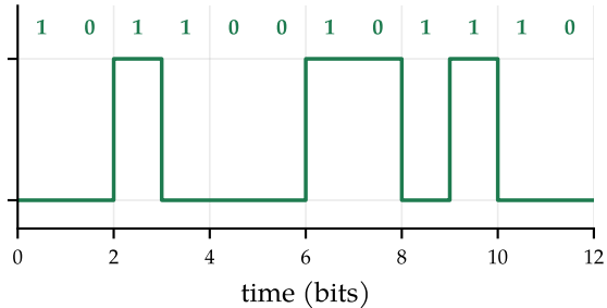
NRZI, wires swapped: every bit right
