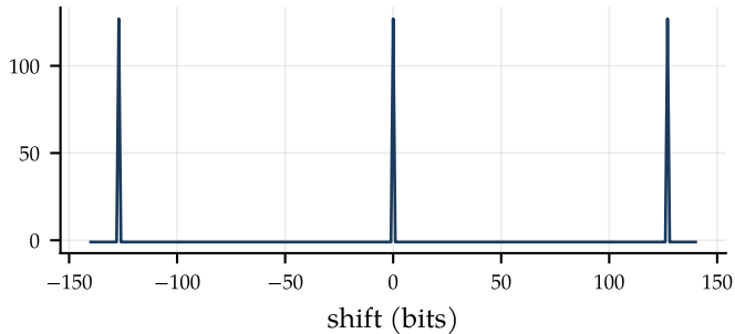
PRBS-7: 127 at zero shift (and every 127 bits), -1 elsewhere
