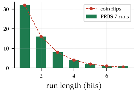
Runs, like coin flips
