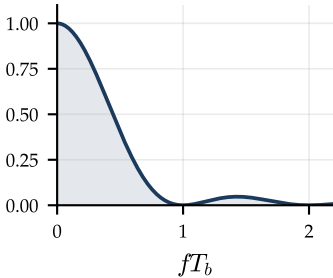
pulse term |P(f)|^2/T
