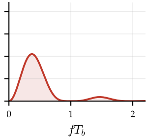
AMI spectrum = product
