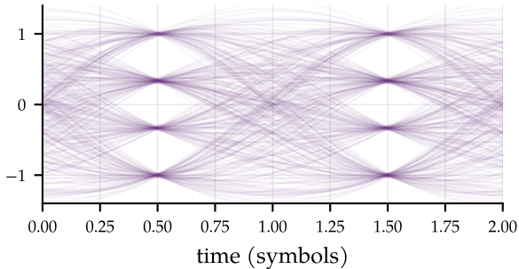
equally spaced levels: three equal eyes
