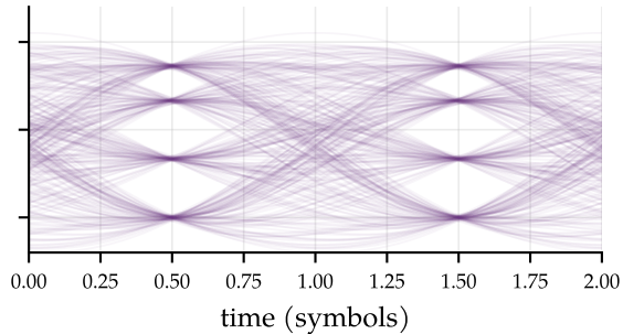
top level compressed: the upper eye shrinks
