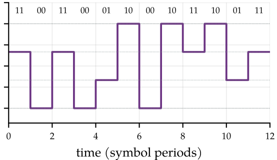
PAM-4: the same 12 symbols carry 24 bits
