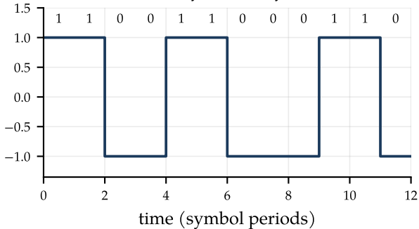
NRZ: 12 symbols carry 12 bits
