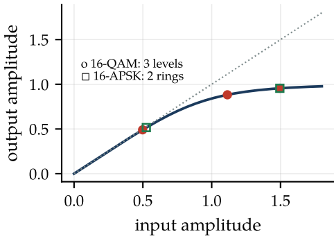
amplifier AM/AM
