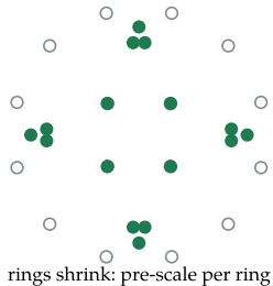
16-APSK after the amplifier
