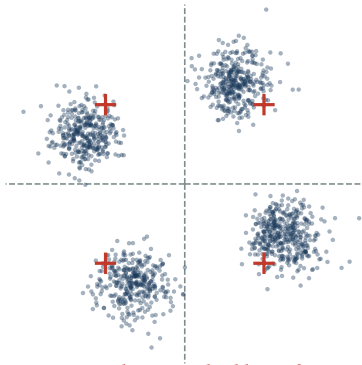
offset = 5% of symbol rate
