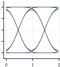
GMSK BT = 0.5
