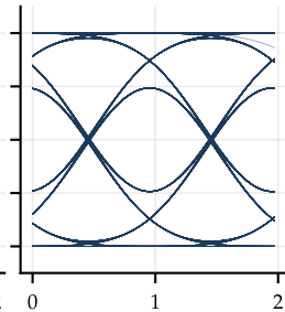
GMSK BT = 0.3
