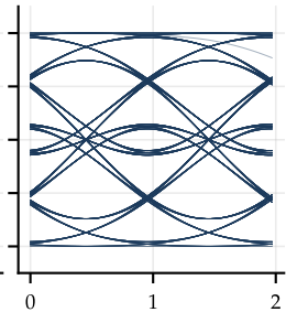
GMSK BT = 0.2
