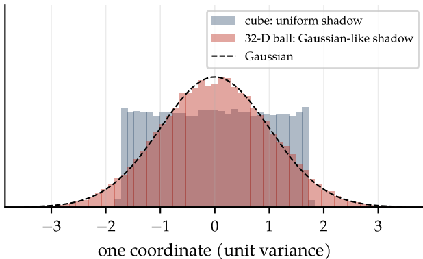
the shadow on one axis
