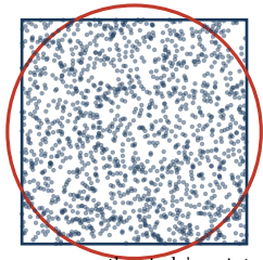
square vs circle in 2-D
