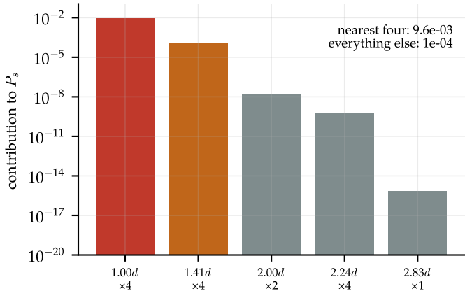
union-bound terms at E_s/N_0 = 16 dB
