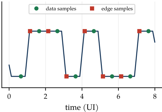
(a) clock late by 0.15 UI: edge = next bit
