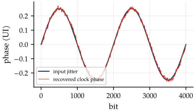
(b) bang-bang loop: slew-limited steps
