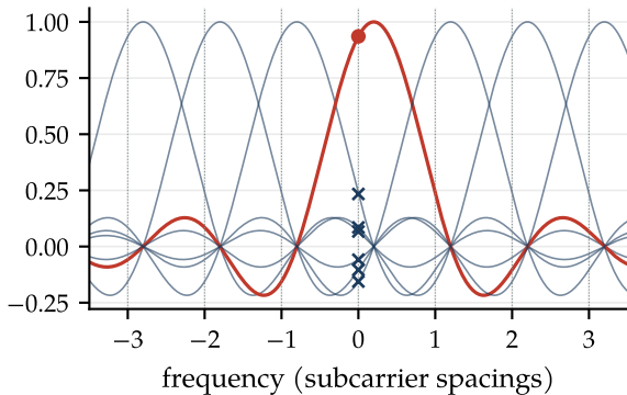
(a) CFO \varepsilon = 0.2 : FFT bins miss the peaks
