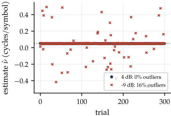
Periodogram, N = 64 , true \nu = 0.05
