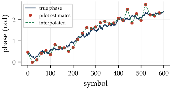
(a) one pilot every 20 symbols
