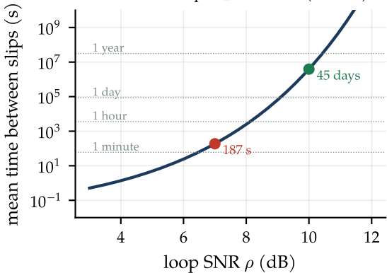
First-order loop, B_L = 100 Hz (Viterbi)
