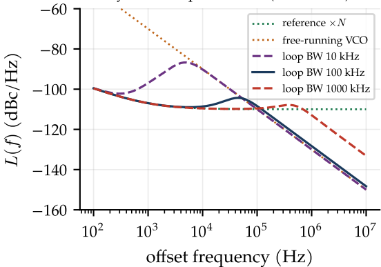
Synthesizer phase noise (illustrative)
