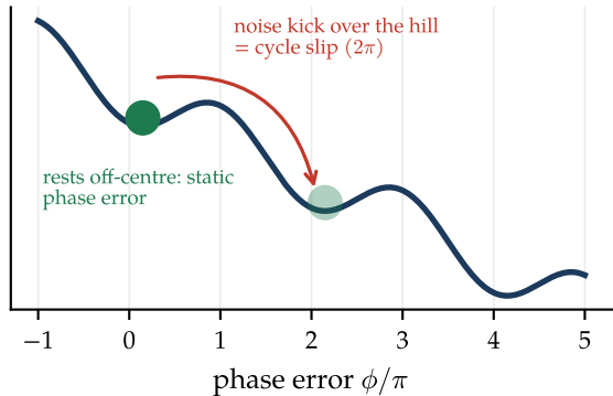
(b) frequency offset tilts the washboard
