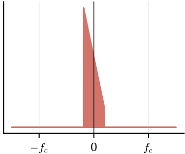
complex envelope \tilde{X}(f)
