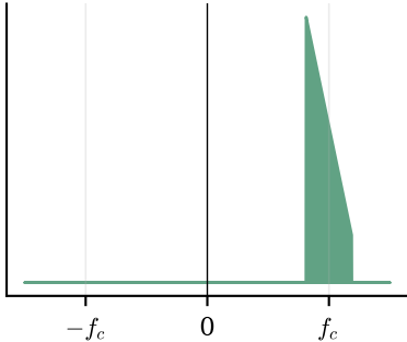
analytic X_+(f)
