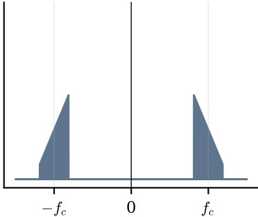
real bandpass X(f)
