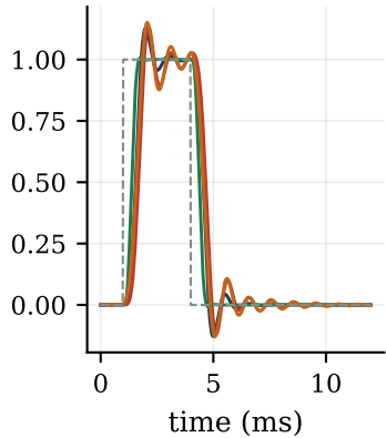
3 ms pulse response
