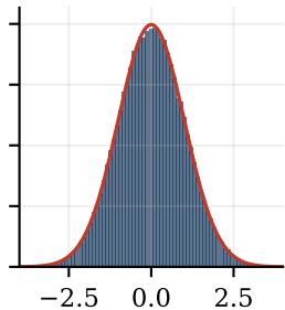
sum of 12 uniforms
