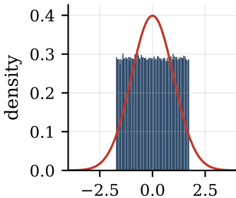
sum of 1 uniform
