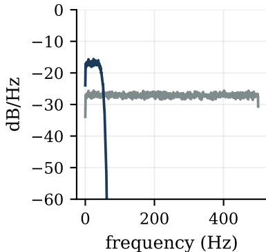
PSD
