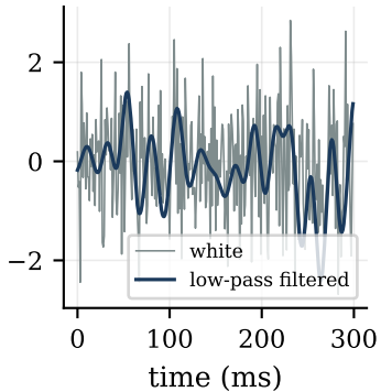
sample paths
