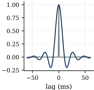
autocorrelation
