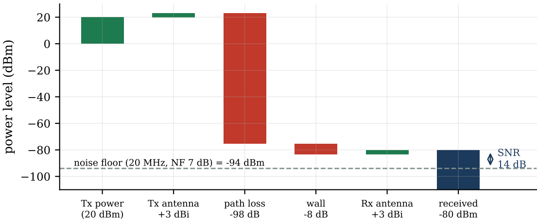
Link budget of an indoor Wi-Fi link as a waterfall
