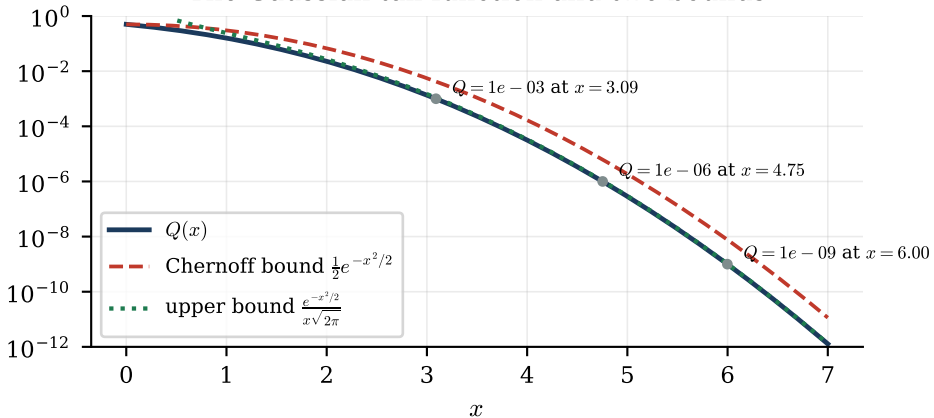
The Gaussian tail function and two bounds
