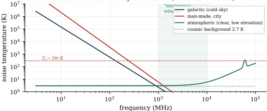
External noise seen by an antenna (illustrative trends)
