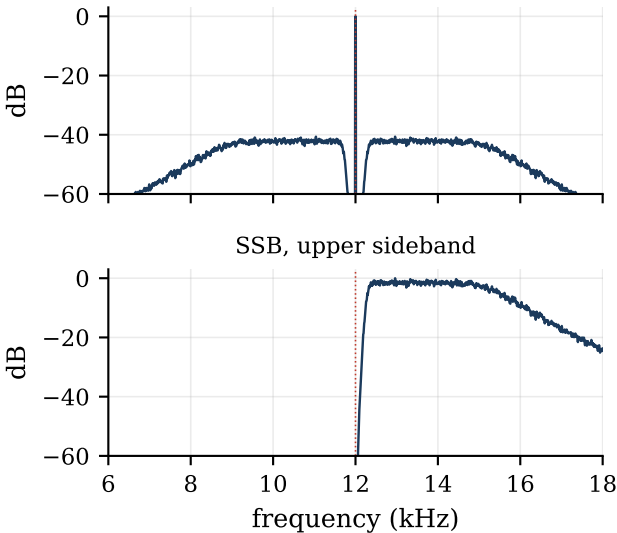
AM (DSB with carrier), \mu=0.8
