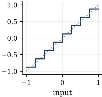
3-bit mid-rise quantizer
