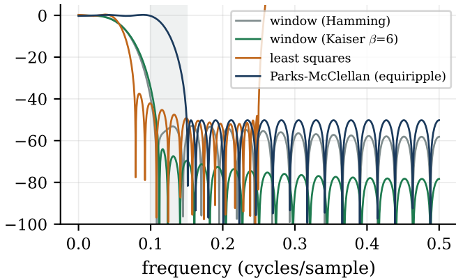
41-tap low-pass designs
