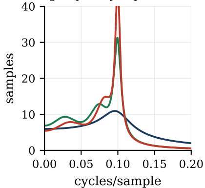
group delay in passband
