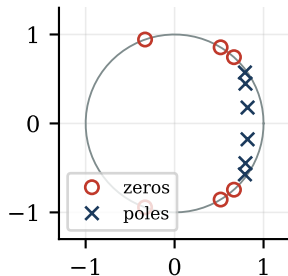
elliptic pole-zero
