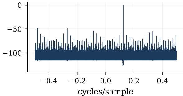
phase truncated to 8 bits
